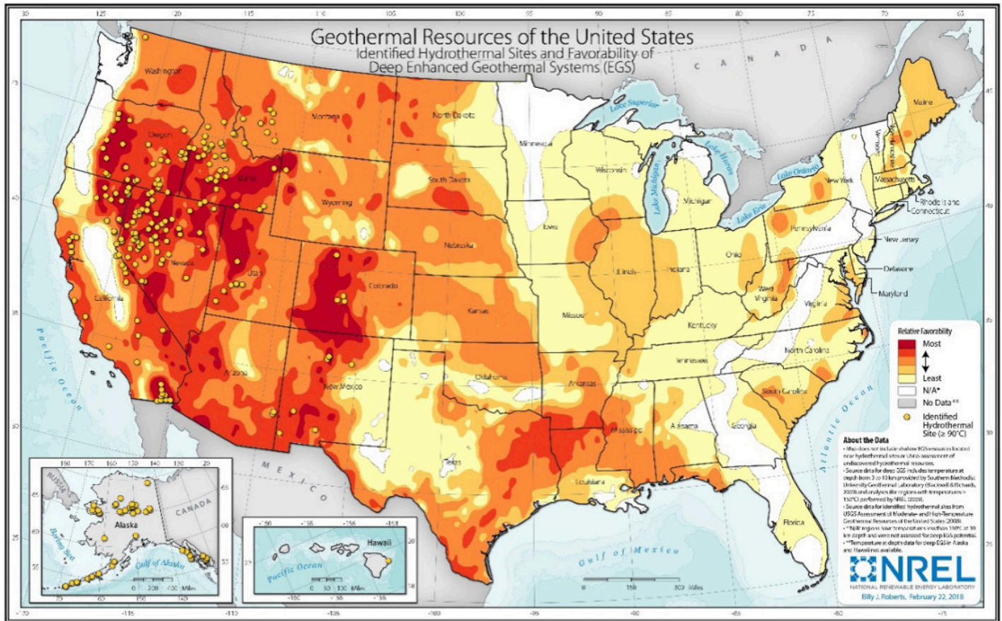
Figure 1: Geothermal Resources map of the United States, from the National Renewable Energy Laboratory, created by Billy J. Roberts (February 22, 2018). https://nrel.gov/gis/geothermal.html
